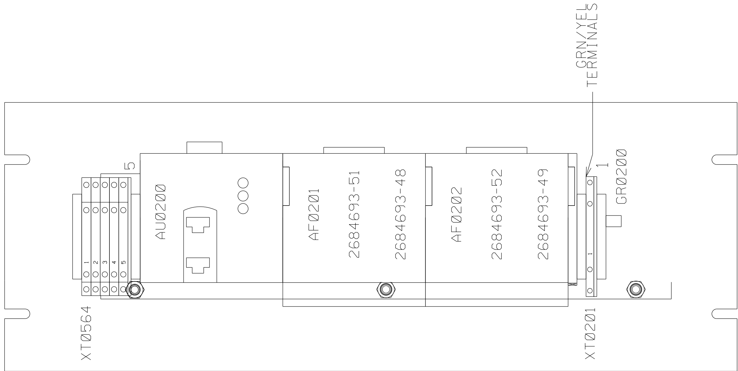
BACK VIEW WITH FLEX I/O INSTALLED TYP. FOR XT0564
